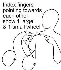
train
